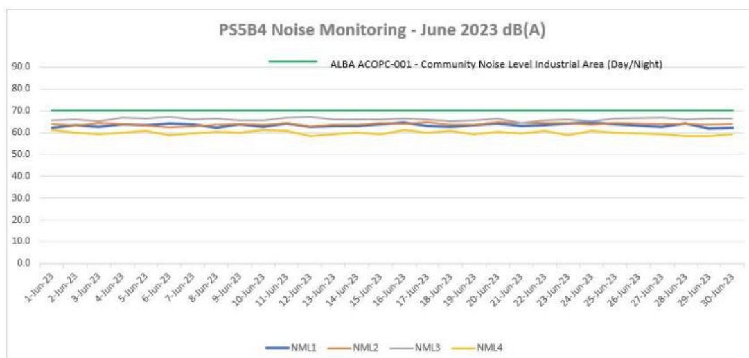
Figure 3.9 Environmental noise levels at receptor locations – June 2023
