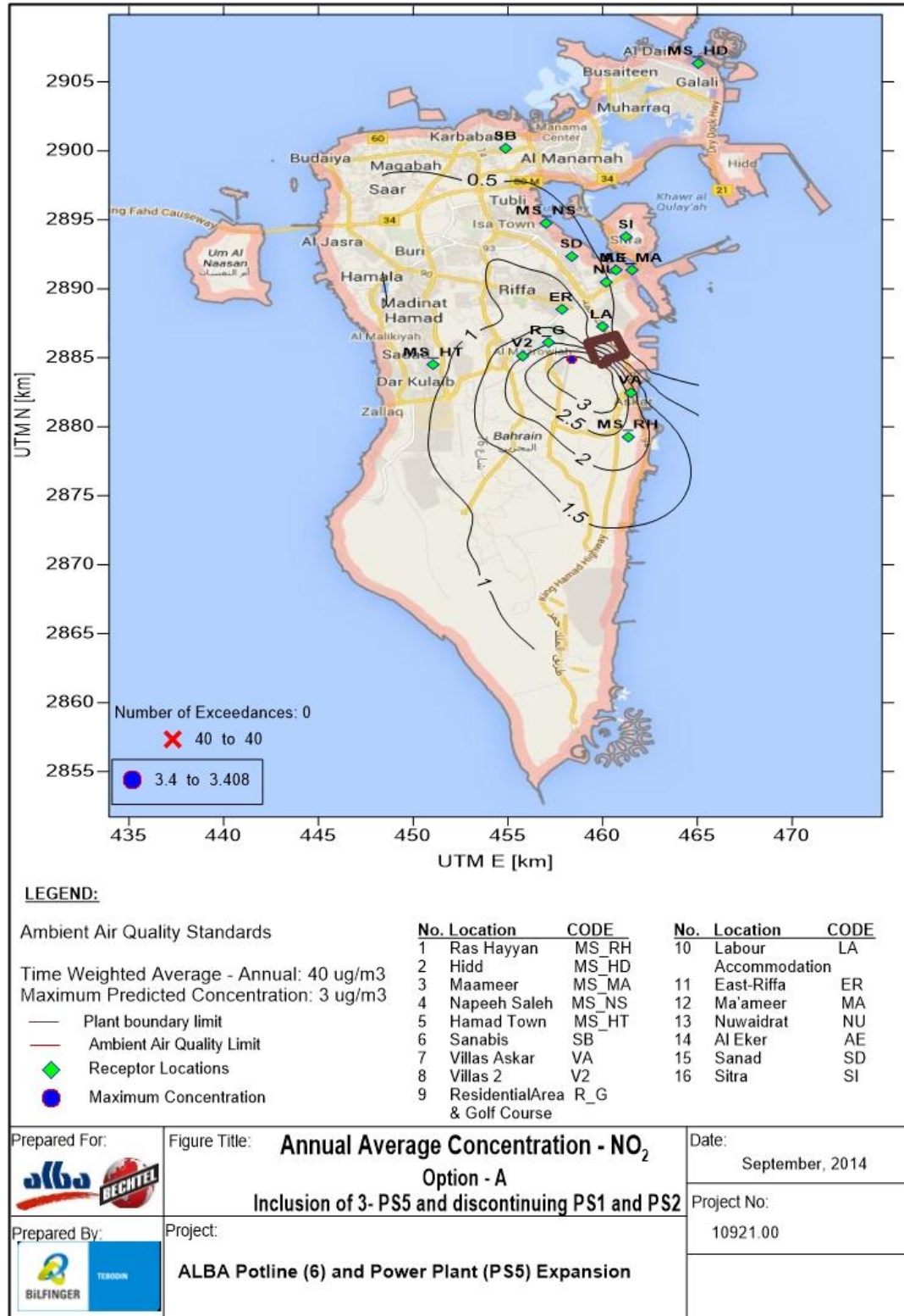
Figure A 6 - Option A- Annual Average Concentration – NO 2
