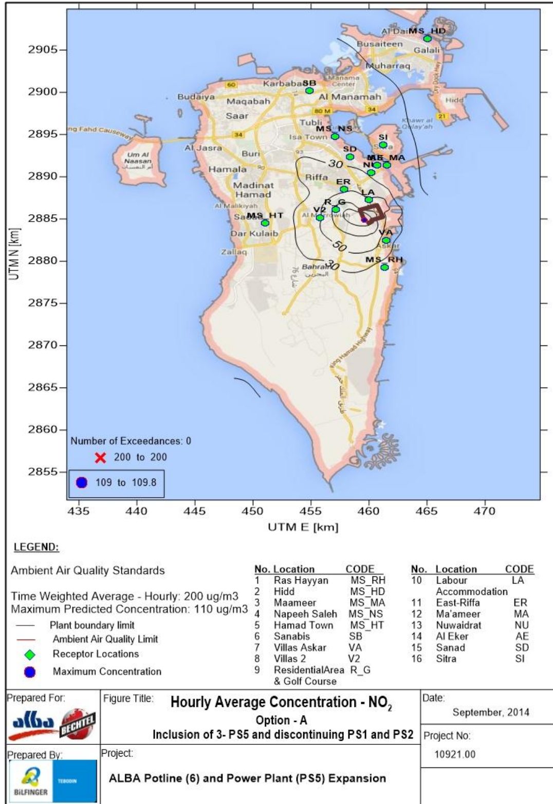
Figure A 4 - Option A- Maximum 1- Hour Concentration – NO 2
