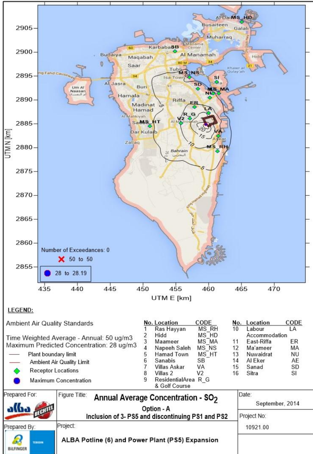
Figure A 3 - Option A- Annual Average Concentration – SO 2
